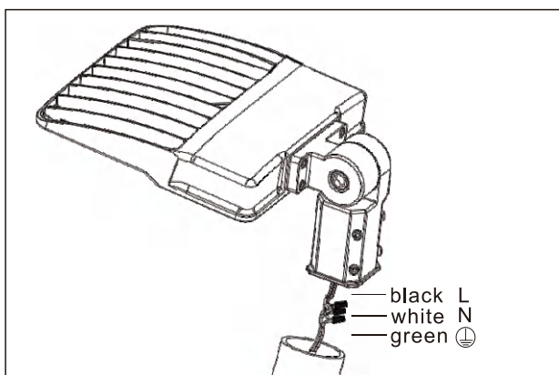
5. Connect wires.
