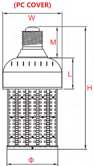
E39 Screw base
