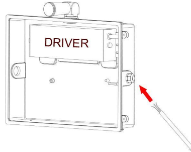
5. Install waterproof connector first, then pass through AC line(pic 5)
